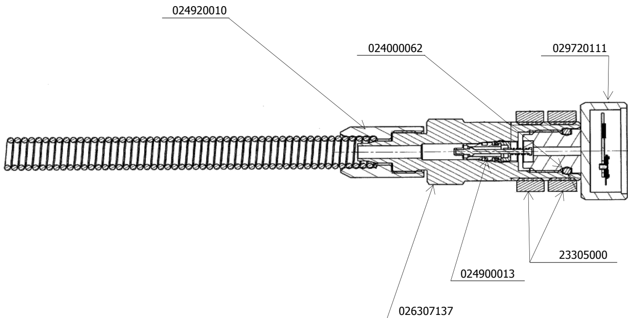
029720111 PRESSURE GAUGE
